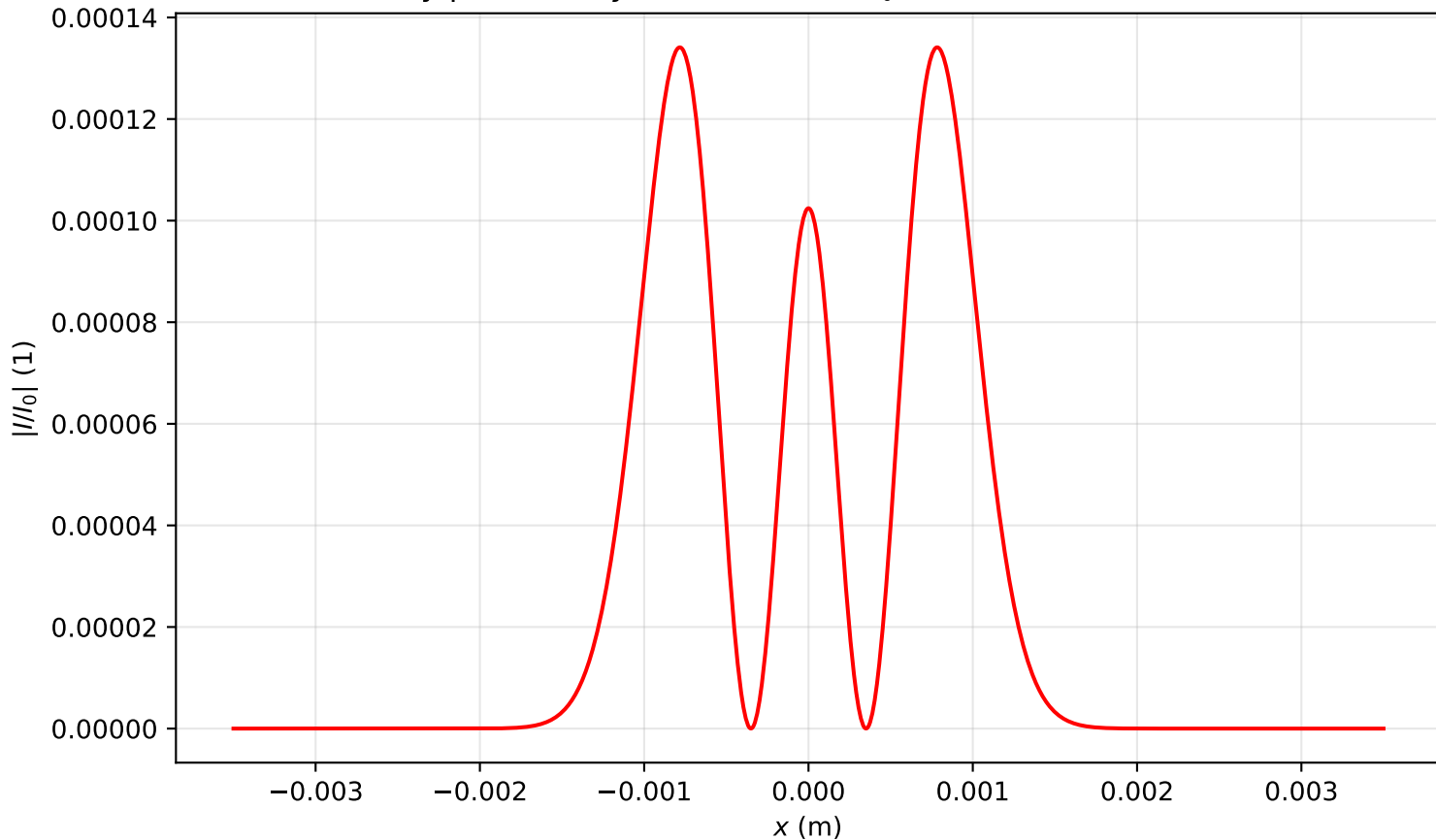
Intensity profile I(x, y = 0, z = 0.080)/I_0 , P_{in}=1.0P_{cr} , artificial time
